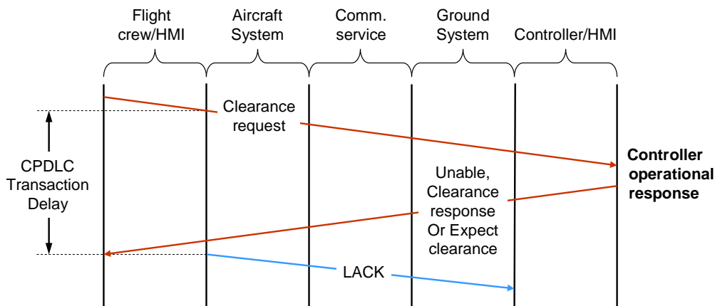
Figure D- 3 Flight crew-initiated ACP delay
