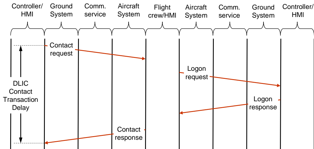
Figure D- 4 DLIC Contact transaction
