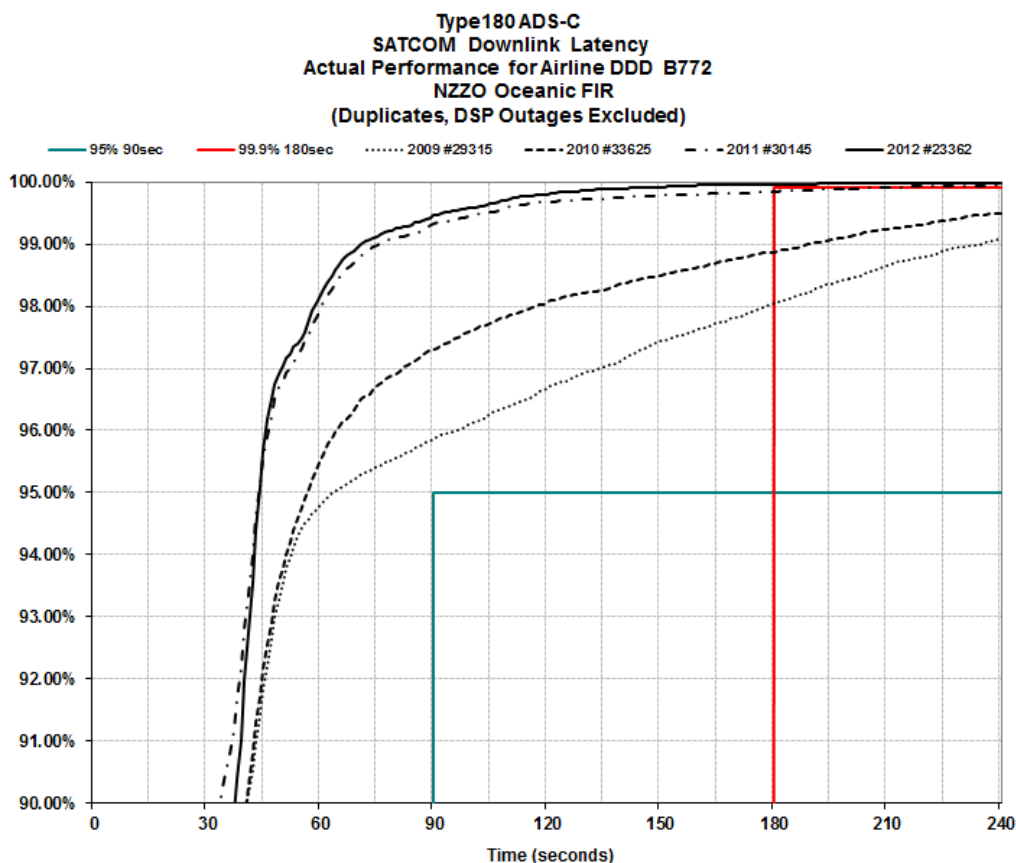
Figure D- 15 SATCOM ADS-C Operator DDD B777 2009-2012
