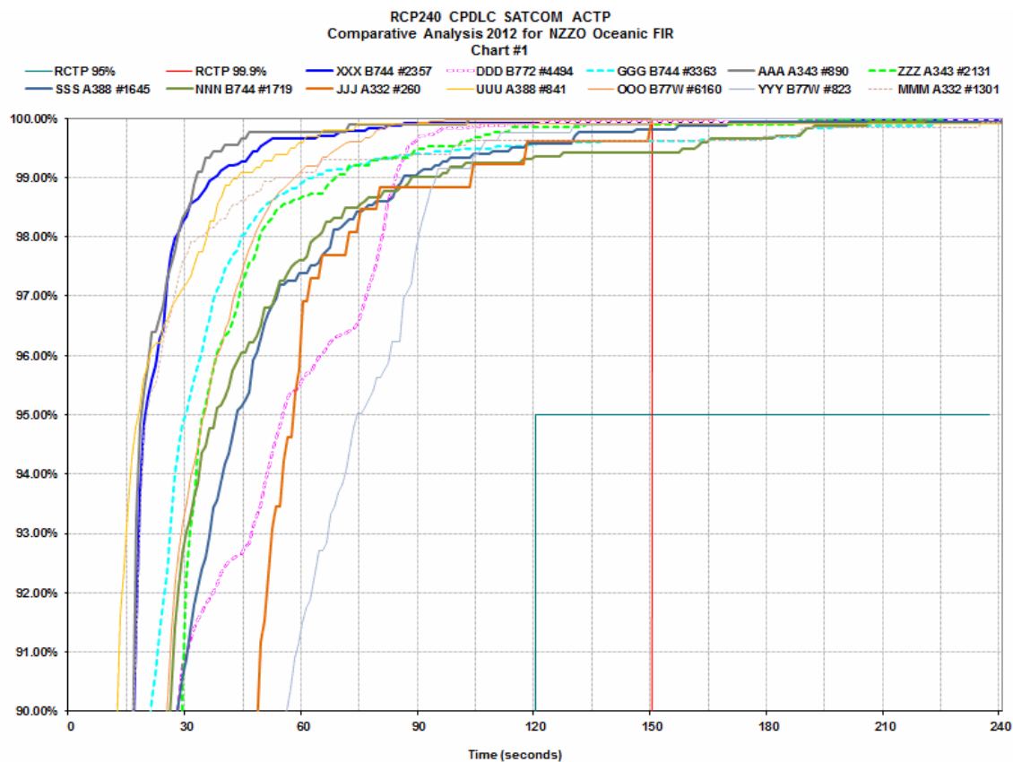
Figure D- 10. CPDLC ACTP comparative operator type performance
