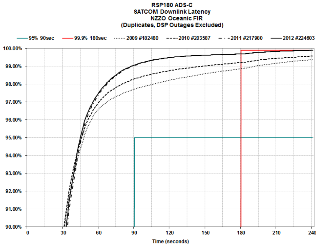
Figure D- 11. ADS-C via SATCOM NZZO FIR 2009 – 2012
