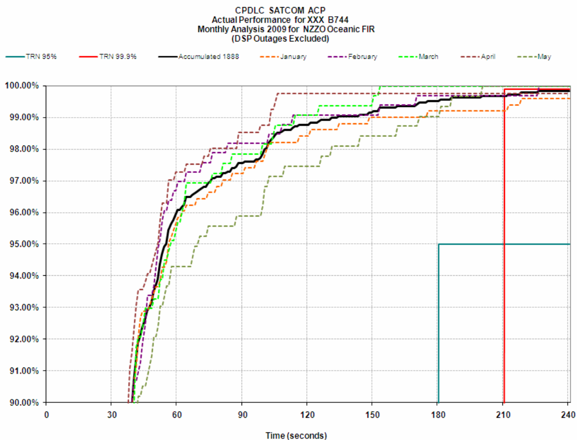
Figure D- 9. Typical Monthly variation in CPDLC ACP
