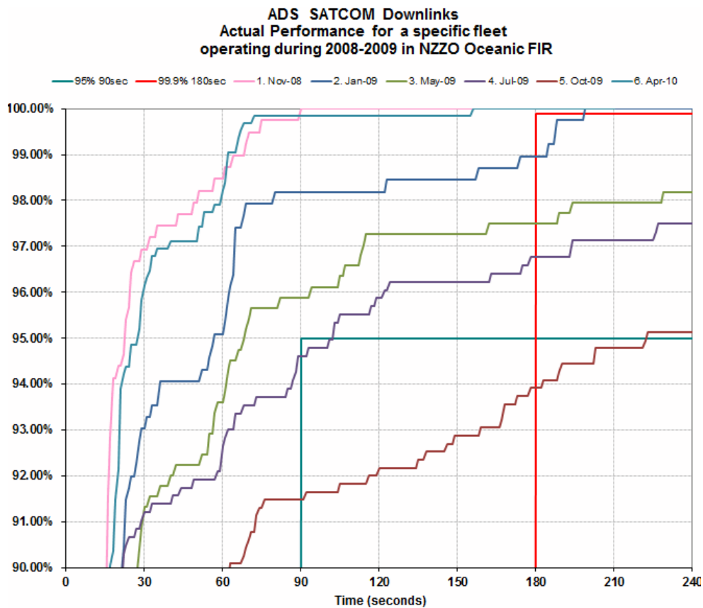
Figure D- 17 Example of ADS-C performance deterioration
