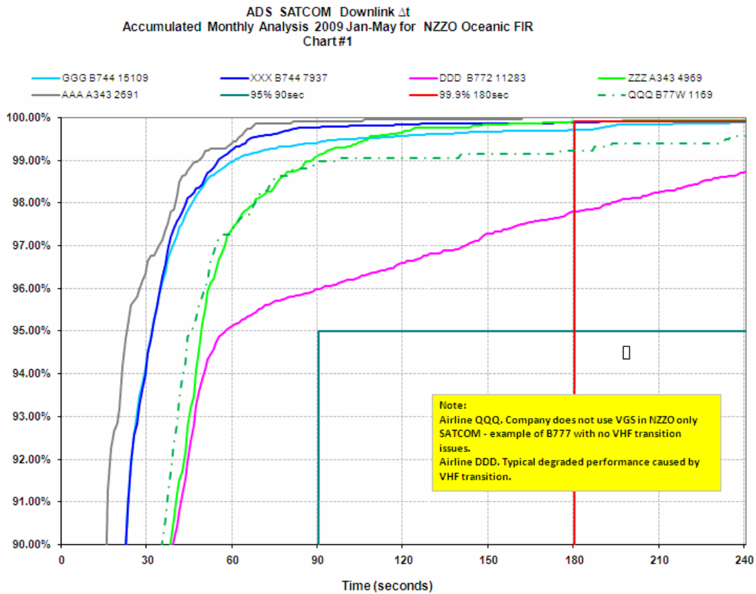
Figure D- 14. Comparative SATCOM ADS-C for different operators
