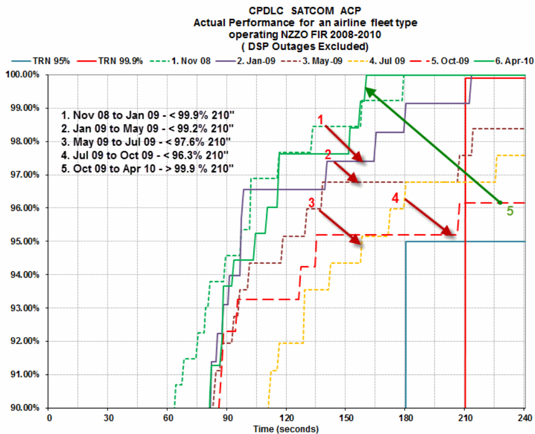
Figure D- 18 Example of CPDLC ACP performance deterioration
