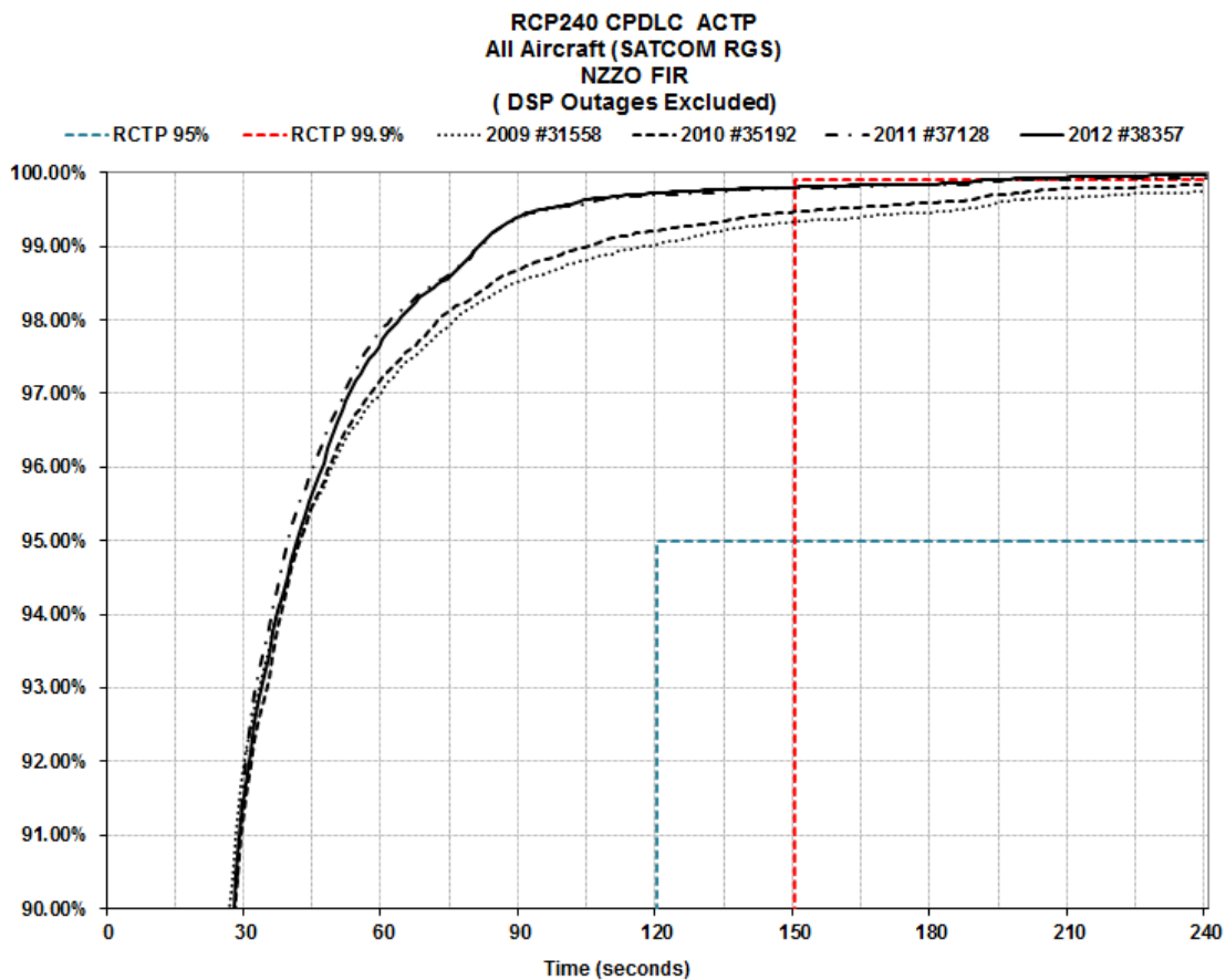
Figure D- 5. CPDLC ACTP performance - Example 1 Graphical by year
