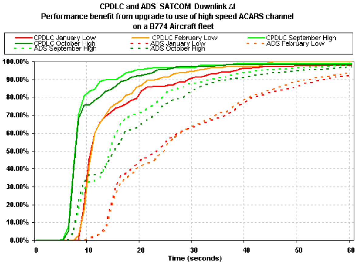
Figure D- 16. Effect of ACARS channel speed on ADS-C surveillance data transit time
