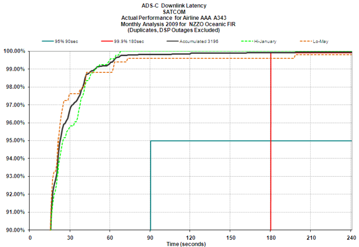
Figure D- 12. ADS-C A343 AAA via SATCOM NZZO FIR Jan – May 2009
