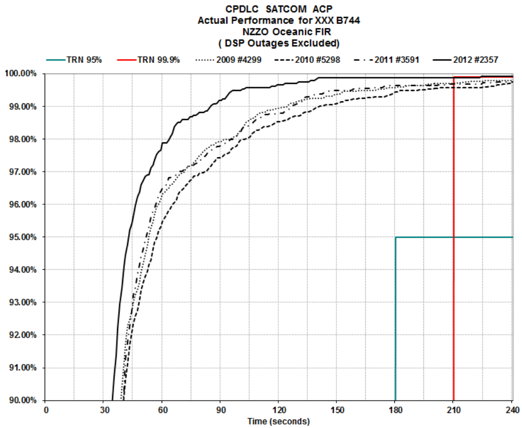
Figure D- 8 CPDLC ACP Airline XXX B744 2009-2012
