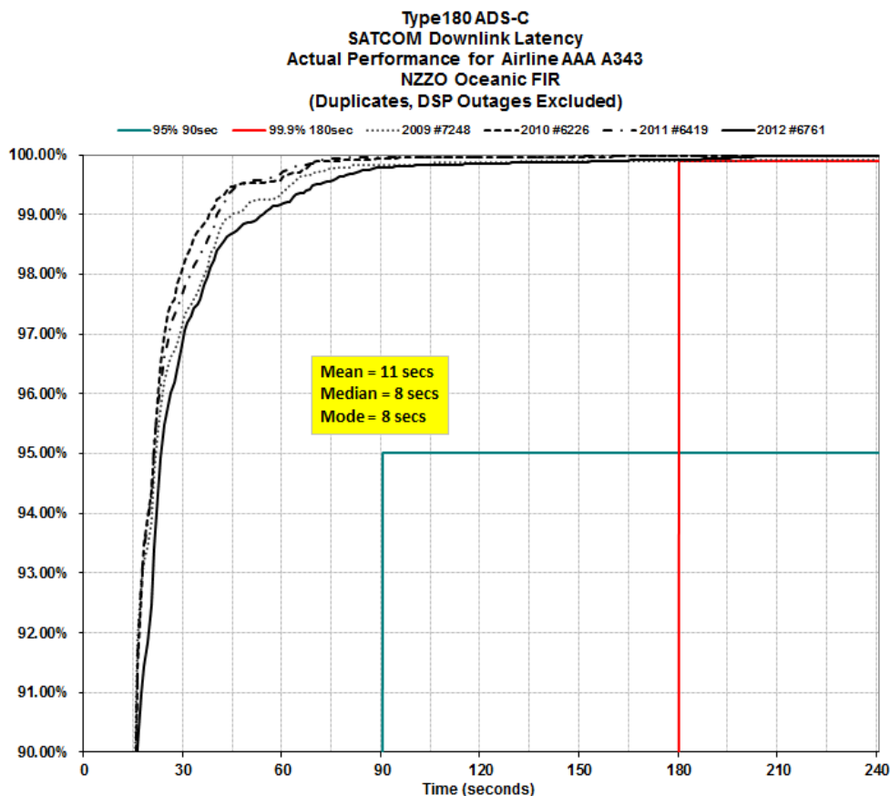
Figure D- 13 ADS-C A343 AAA via SATCOM NZZO FIR 2009-2012
